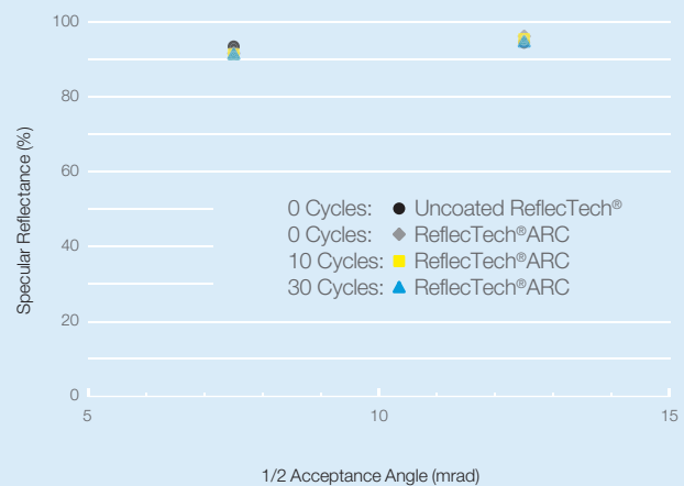
Figure 2. Abrasion resistance of ReflecTech®ARC in terms of Taber abraser cycles with 250 g arm weight. Specular reflectance was measured at 660 nm, and \theta = 7.5 and 12.5 mrad half acceptance angles.
