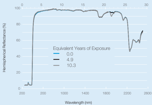
Figure 3. Spectral hemispherical reflectance of ReflecTech®ARC samples after 0 (initial), 4.9, and 10.3 years' equivalent UV exposure in NREL's UAWS. Samples exposed at 30°C.
